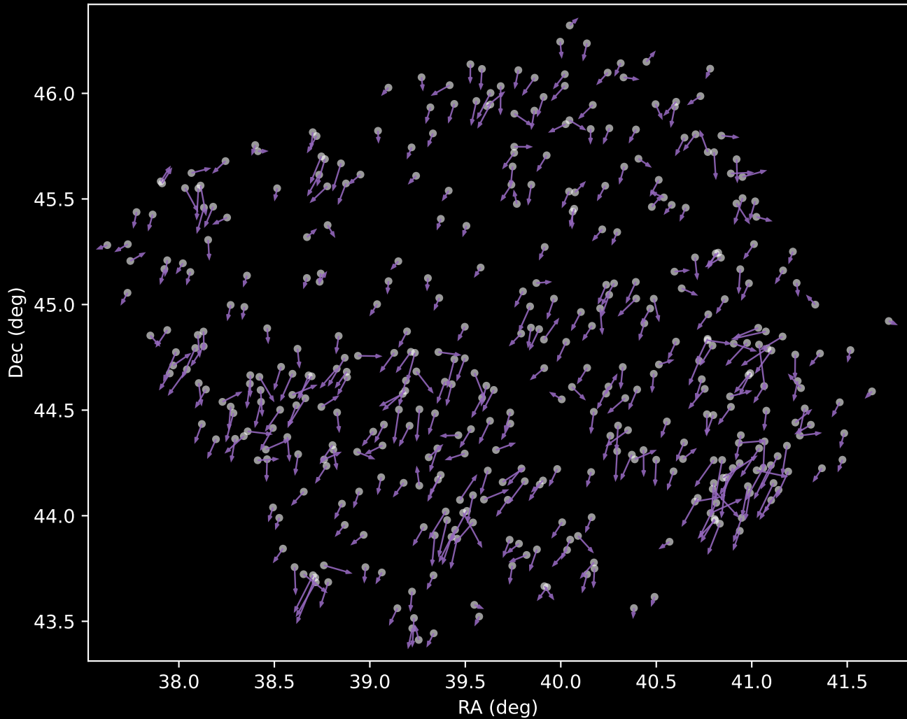
APOGEE DR17 Cluster 8 Proper Motion Vectors (n=413)
