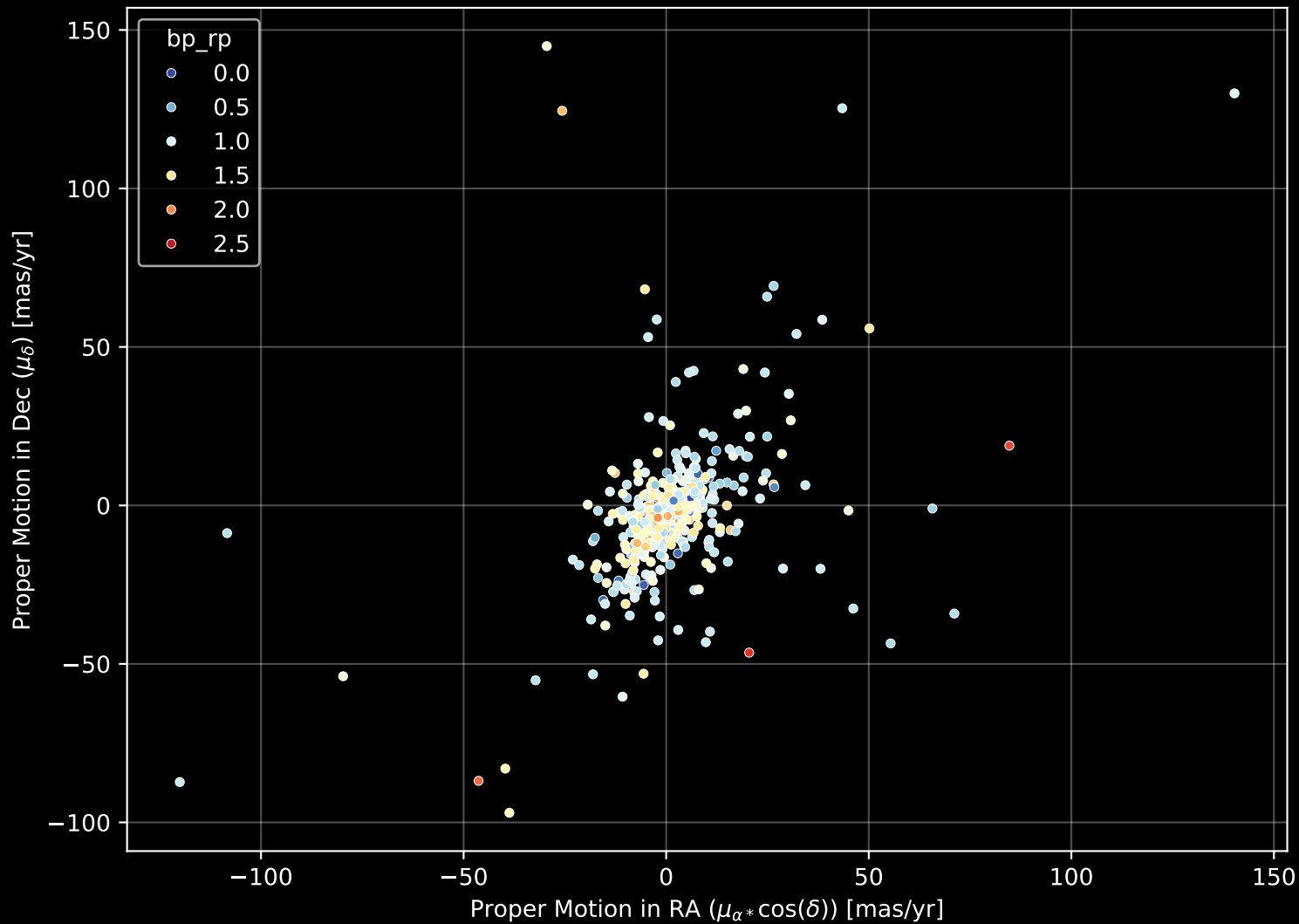
APOGEE DR17 Field: [K14_080+08] Proper Motion Diagram (n= 704)
