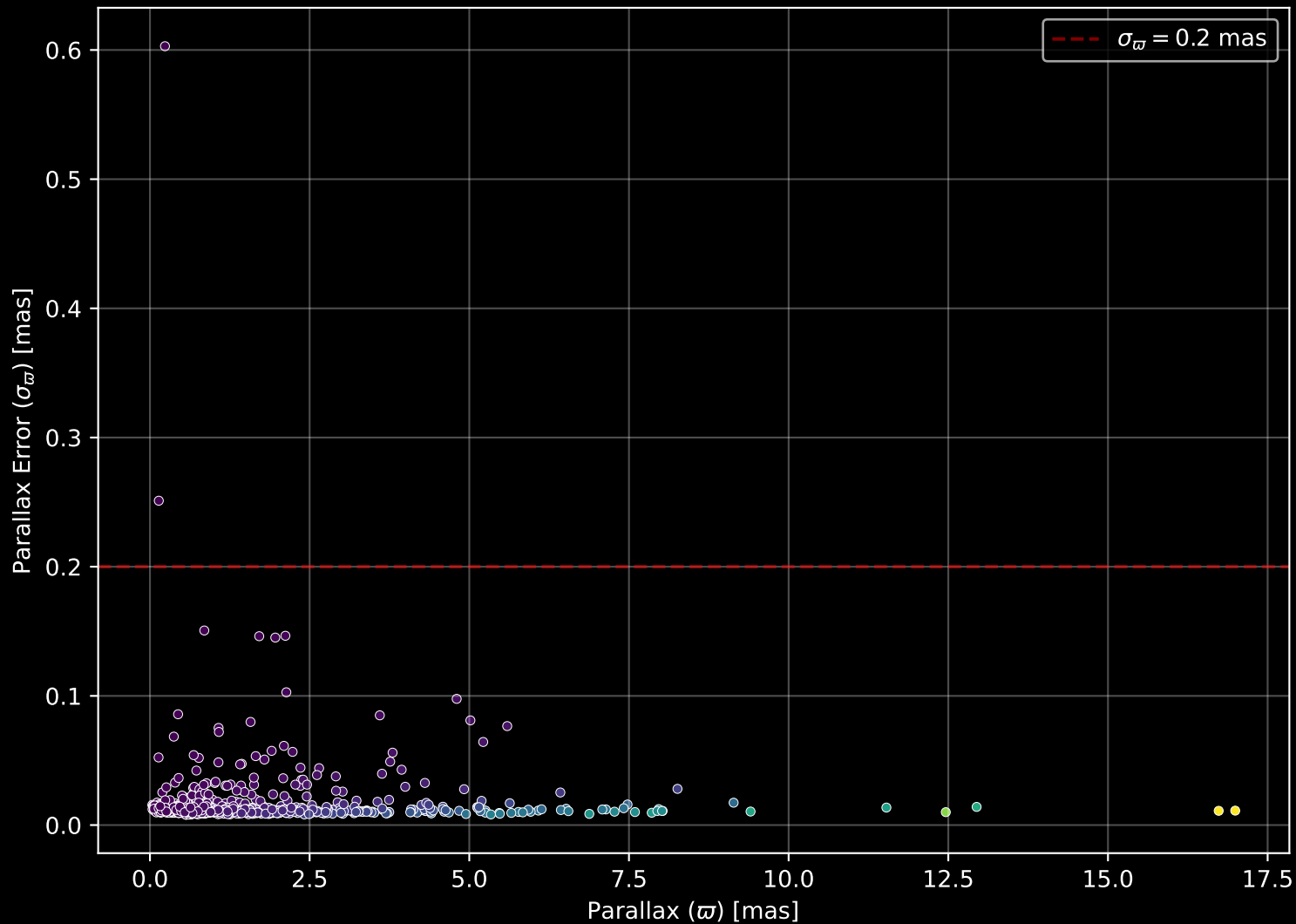
APOGEE DR17 Field: [K14_080+08] Parallax Quality (n= 704)
