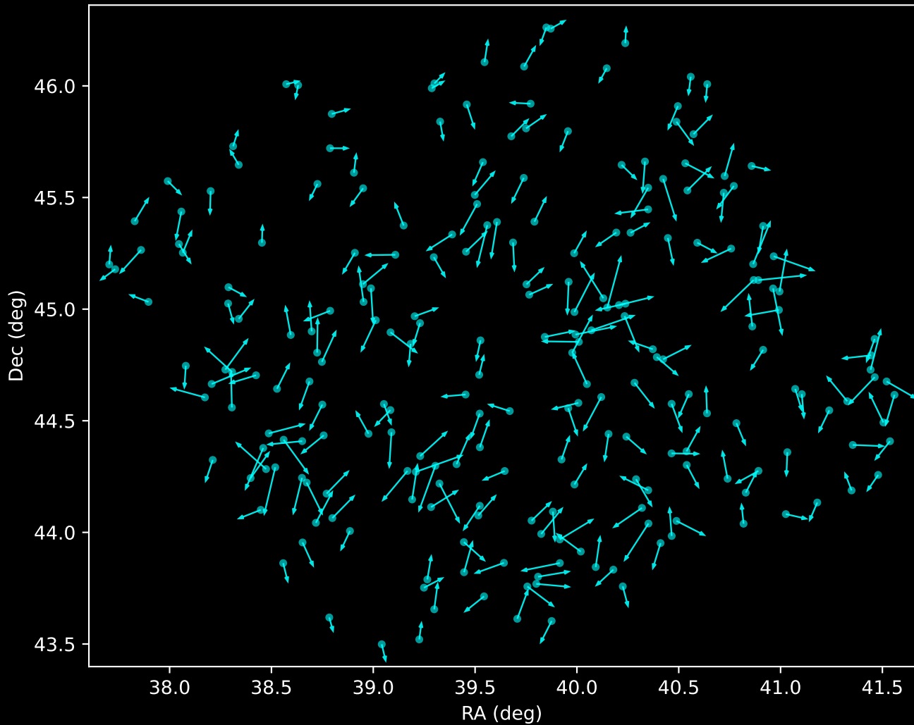
APOGEE DR17 Noise Stream Proper Motion Vectors (n=231)
