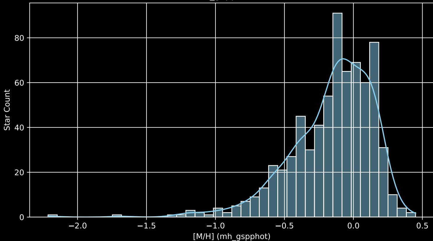
APOGEE DR17 Field: [K14_080+08] [M/H] (mh_gspphot) (n= 701)
