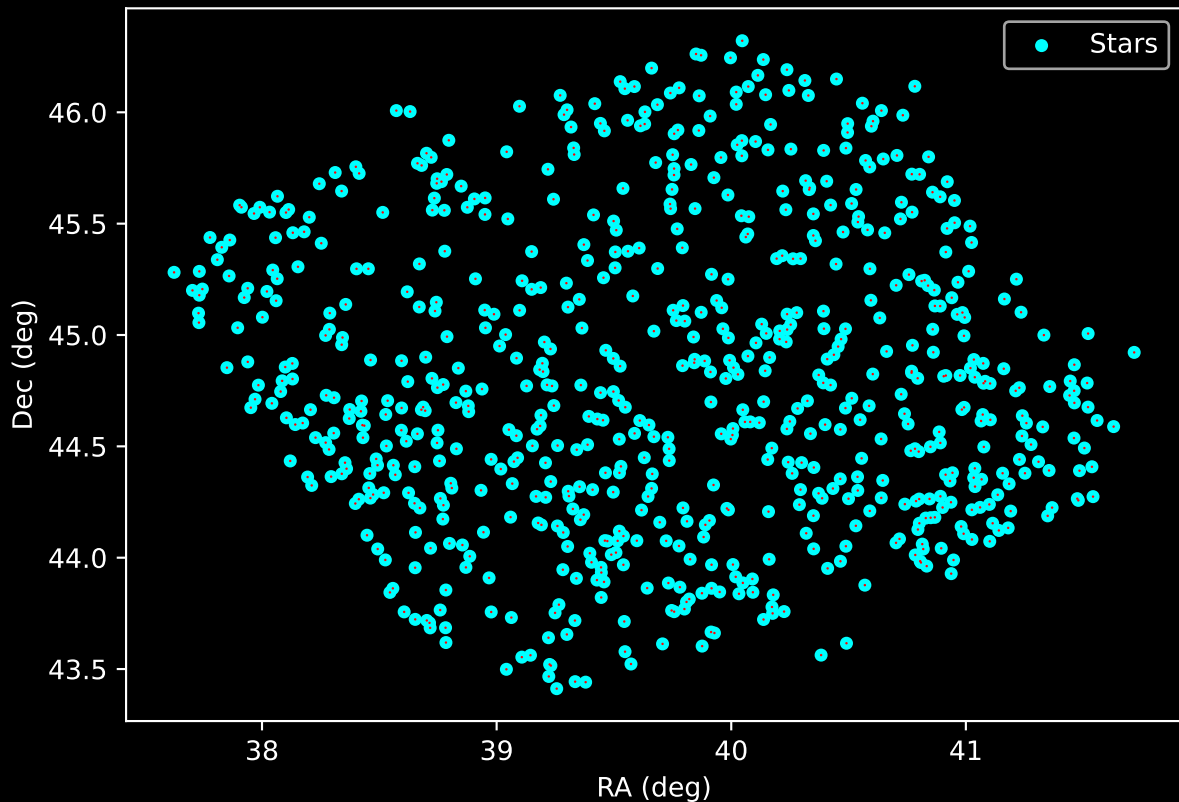
APOGEE DR17 Field: [K14_080+08] Proper Motion Vectors for Gaia Star Field (n= 704)
