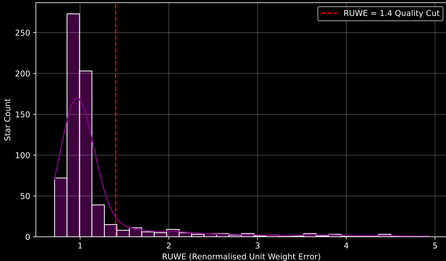
GAPOGEE DR17 Field [K14_080+08] RUWE Distribution (n= 685)
