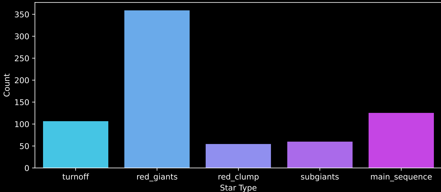
APOGEE DR17 Field: [K14_080+08] Count plot of Star Type
